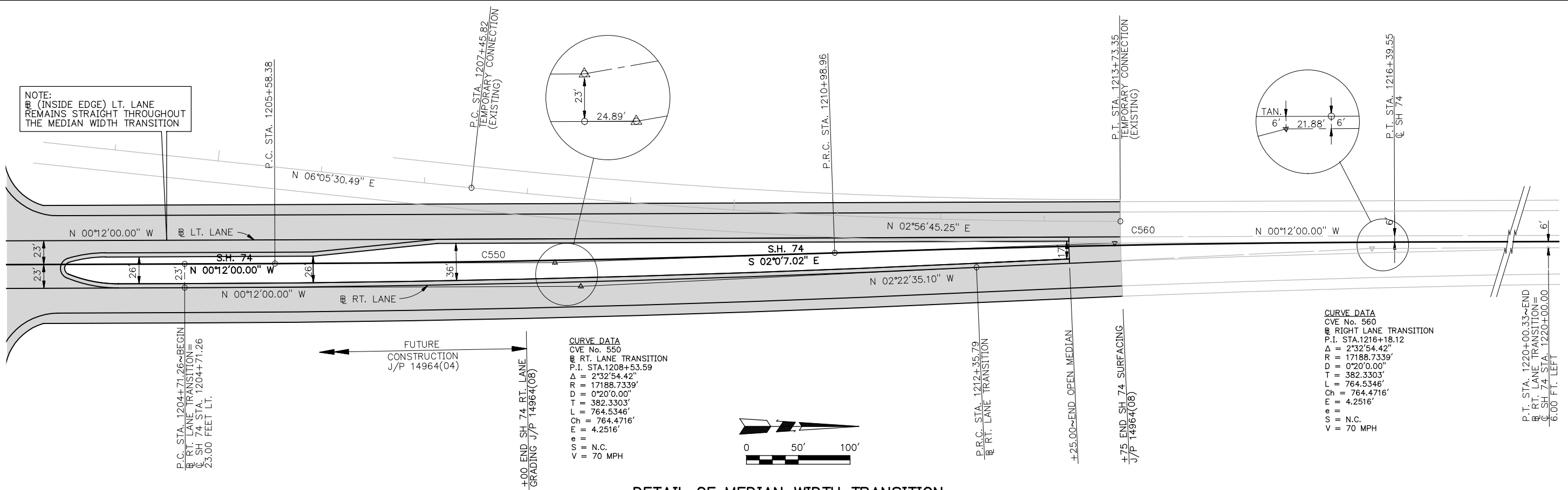
DETAIL OF MEDIAN WIDTH TRANSITION
