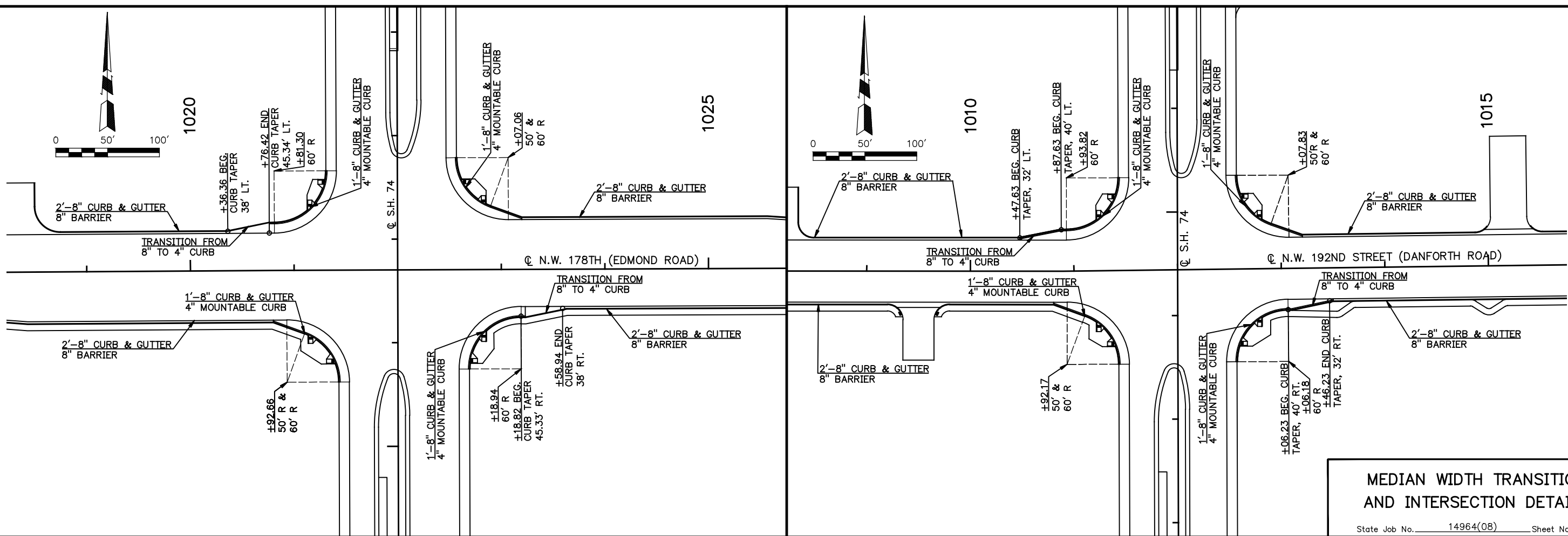
DETAIL OF MEDIAN WIDTH TRANSITION
